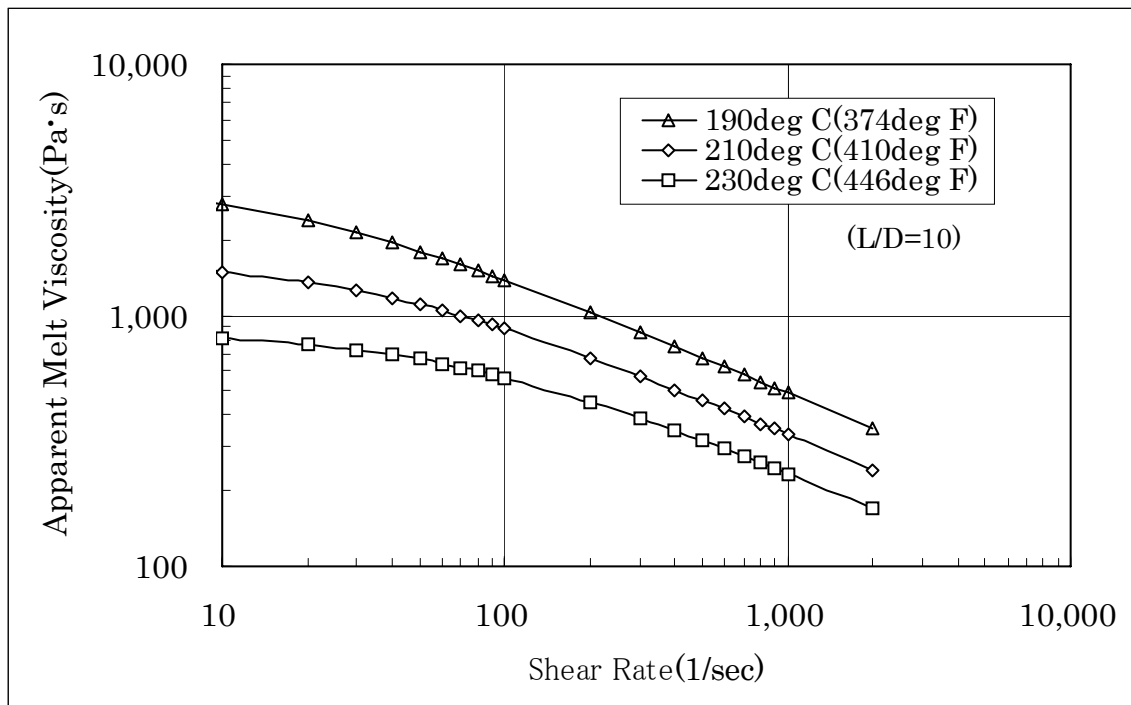
Fig.1 Melt Viscosity of Soarnol A4412 B
