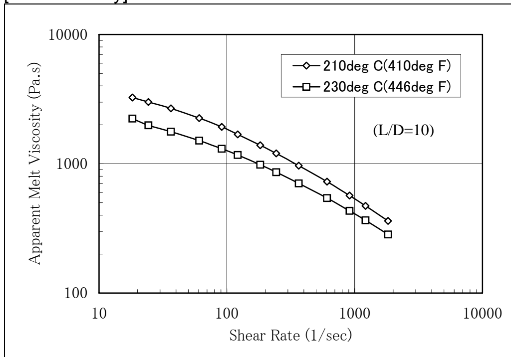
Fig.1 Melt Viscosity of Soarnol DT2904RB
