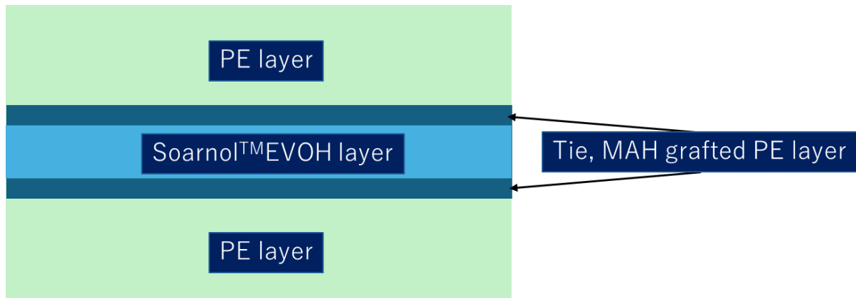
Figure 1. 'PE based barrier film with SoarnoL™ EVOH and PE-g-MAH' technology by Mitsubishi Chemical Europe GmbH.
